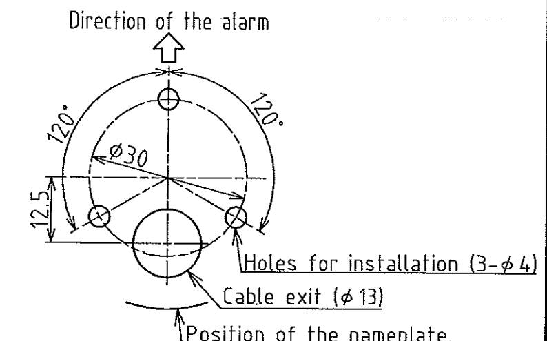
Dimension of installation surface (For direct mount)
