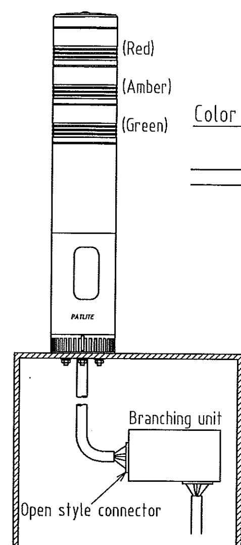
Installation example
