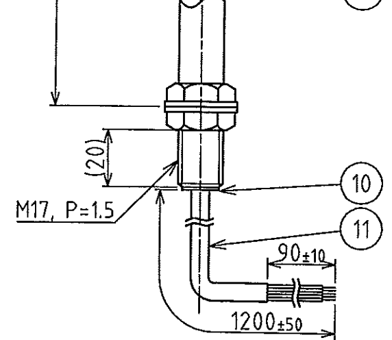
LE-D3(B)P Pole mount type
