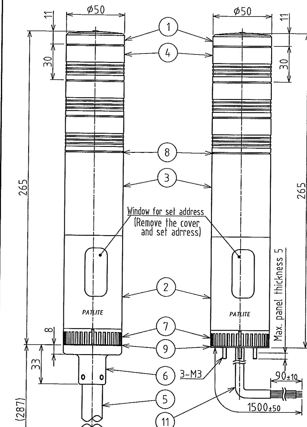
LE-D3(B)W Direct mount type
