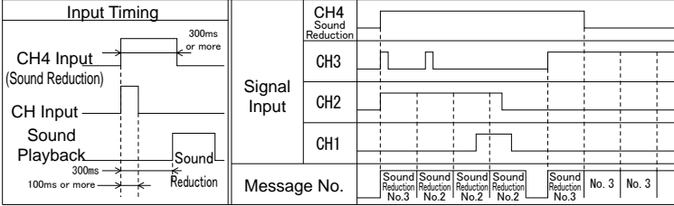
Sound Reduction Timing Chart (Bit Input)
