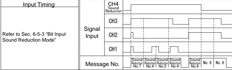
Sound Reduction Timing Chart (Binary Input)
