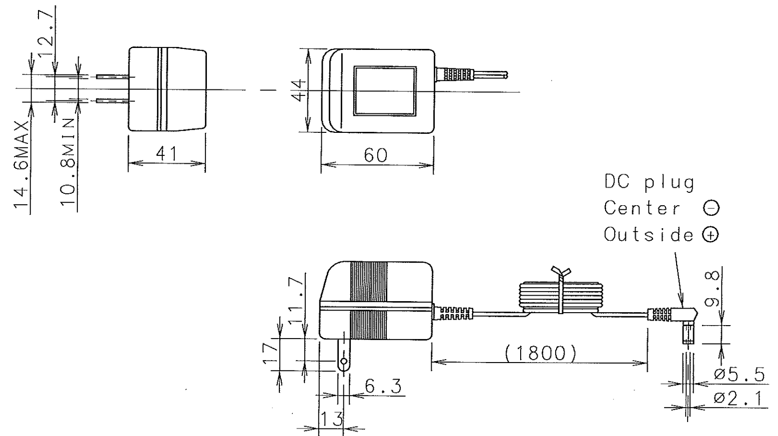
AC adapter
