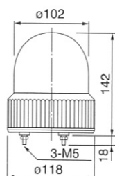
Mounting Dimensions
