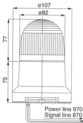
Mounting Dimension
