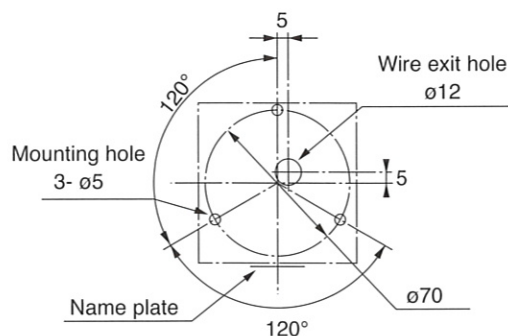
Mounting Dimension
